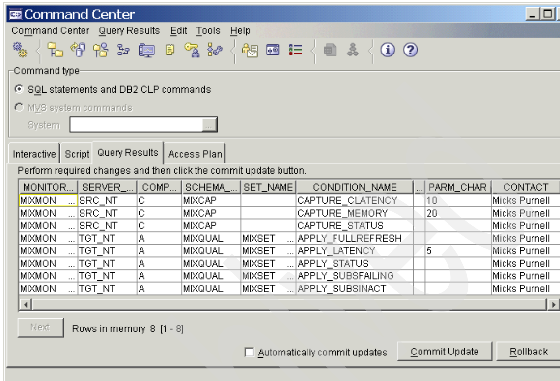
Figure 7-7 Monitor conditions displayed in Command Center
