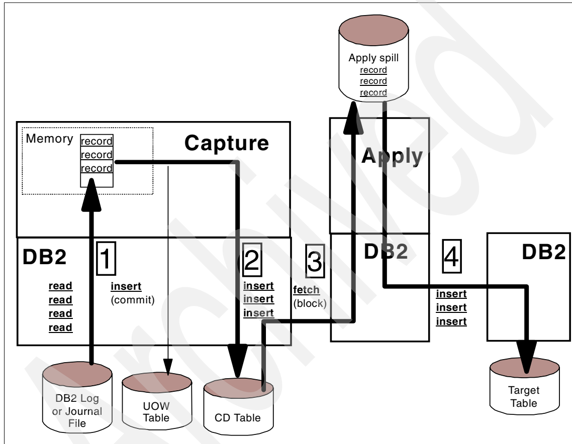
Figure 10-2 Replication - push system design
