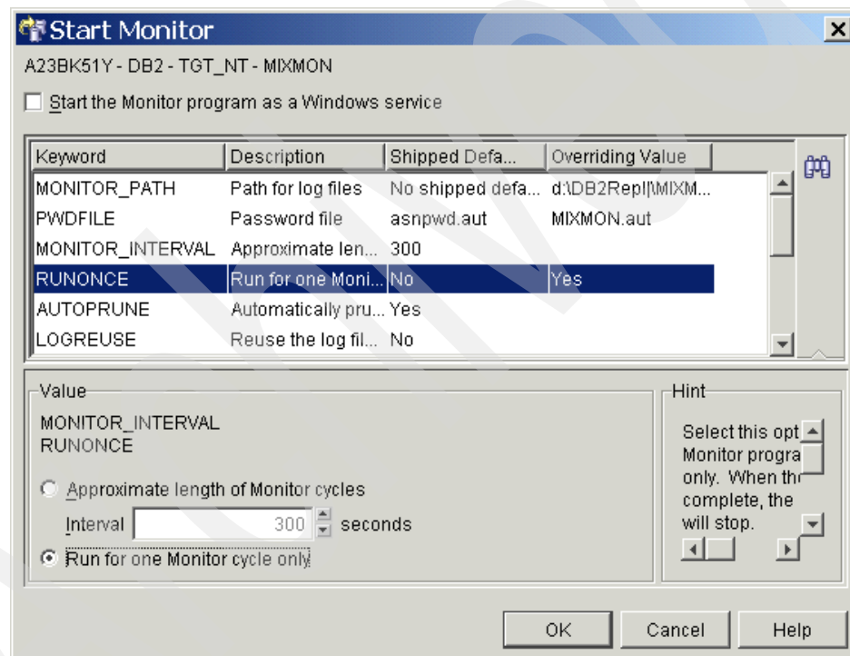
Figure 7-8 Start Monitor window example in Replication Center
