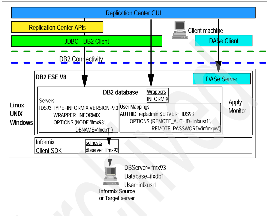
Figure 2-7 Federated Server configuration example to Informix
