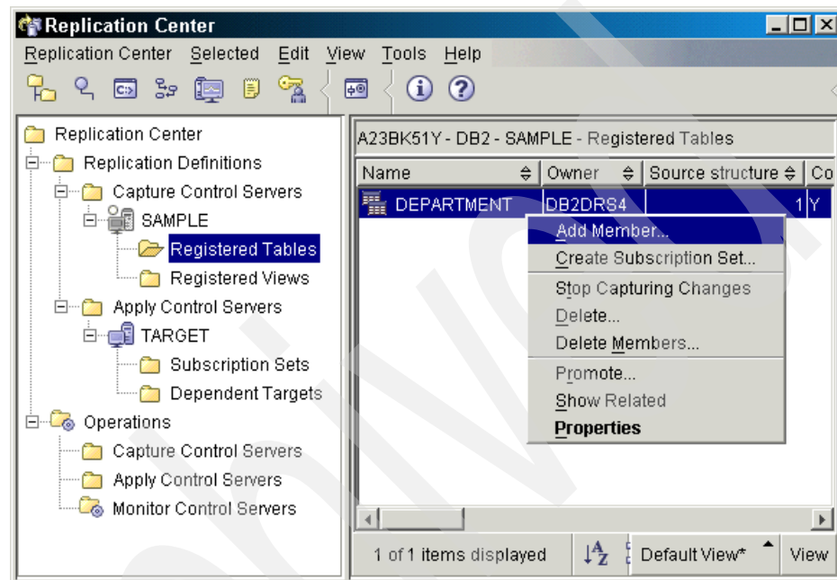
Figure 2-14 Expanded tree with objects and options
