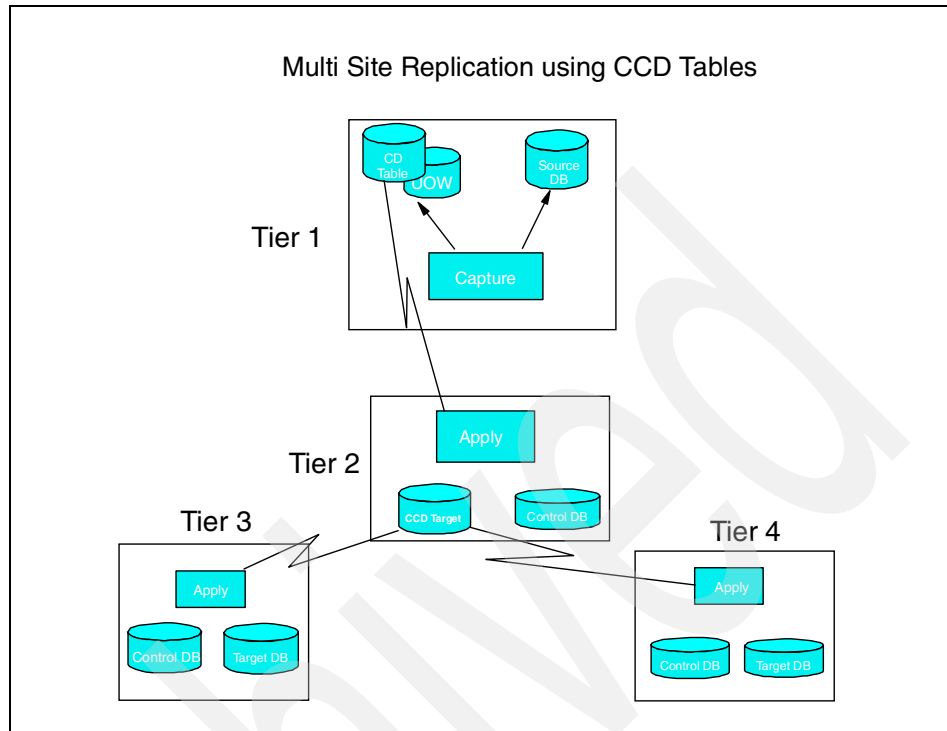
Figure 5-20 CCD table multi tier replication
