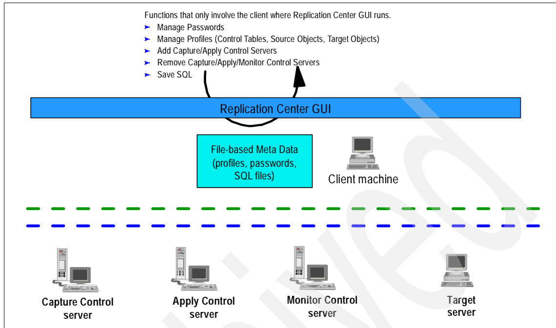
Figure 2-5 Access to profiles, passwords, and SQL files
