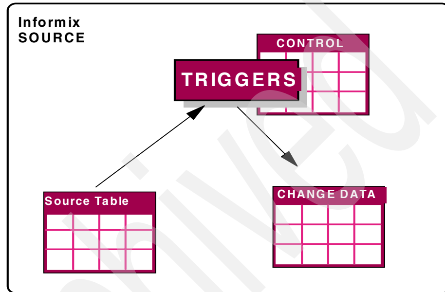
Figure 1-8 Capture for Informix
