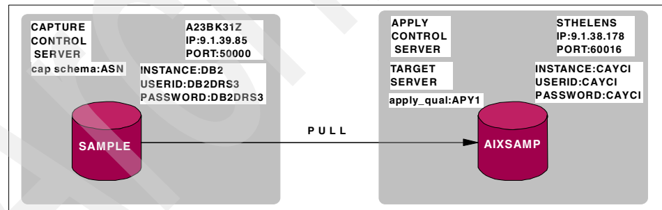
Figure 6-5 Sample replication configuration on Windows and AIX
