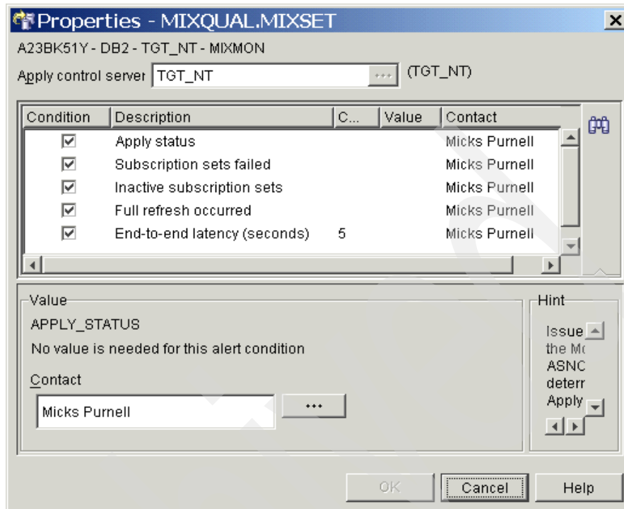
Figure 7-6 Alert conditions for Apply
