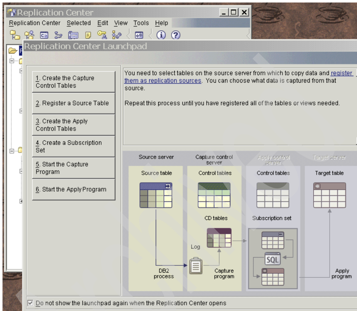
Figure 2-10 Replication Center and Replication Center Launchpad
