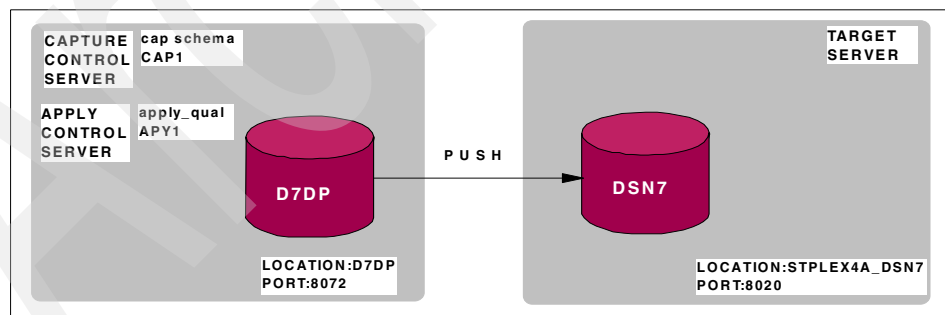
Figure 6-20 Sample replication configuration for z/OS to z/OS
