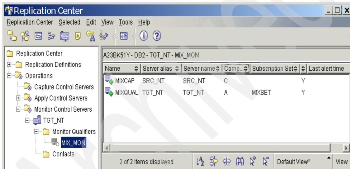
Figure 7-5 Capture and Apply alert entries in Replication Center
