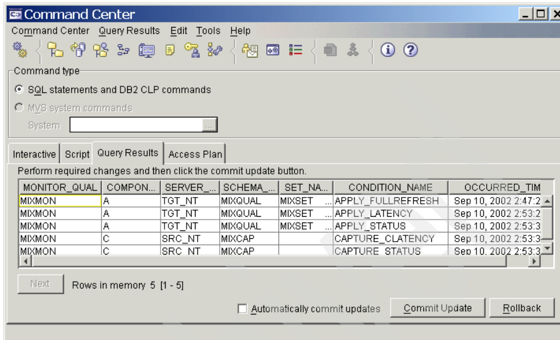
Figure 7-11 Replication alert records in the ASN.IBMSNAP_ALERTS table
