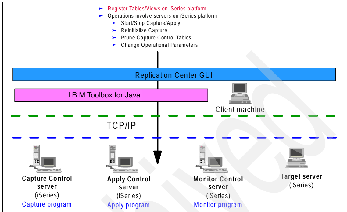
Figure 2-4 Use of IBM Toolbox for Java API's to iSeries servers
