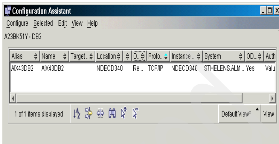
Figure B-6 Configuration Assistant - DB2 on Linux or UNIX connection entry
