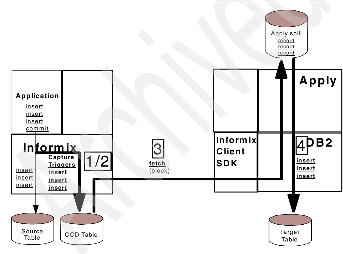
Figure 10-5 Replicating from Informix - pull system design
