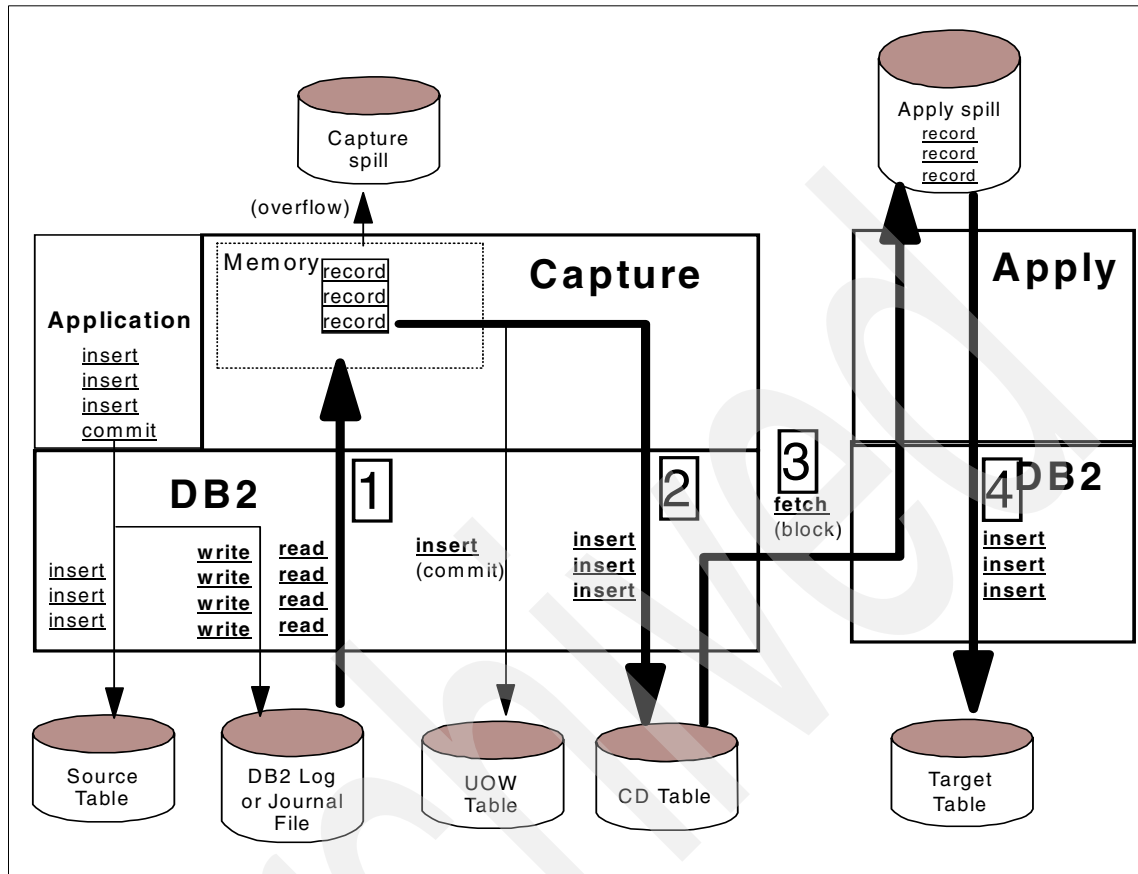
Figure 10-1 Replication - 'pull' system design
